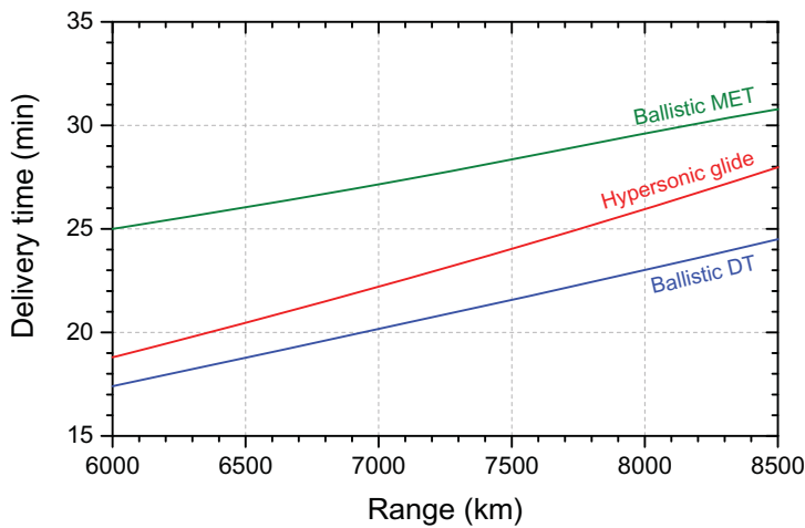
Figure 8. Calculated total delivery times for a hypersonic missile and a ballistic missile flying both minimum energy and depressed trajectories. Delivery times include boost, ballistic, reentry, pull-up, glide, and terminal phases, where applicable. Ballistic missiles fired on depressed trajectories reach their targets most quickly. Their delivery time advantage over hypersonic gliders increases with range.
